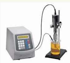
Ultra Probe Sonicator Probe sonicator with optional sound enclosures
